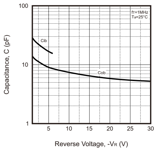
Fig.5 - Cib/Cob — VEB/VCB
