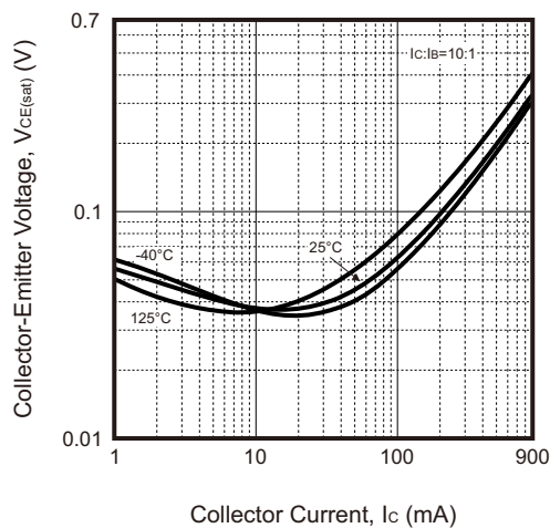
Fig.8 - Collector-Emmitter Saturation Voltage
