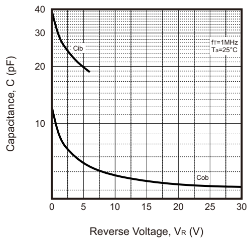
Fig.10 - C ib /C ob — V EB /V CB
